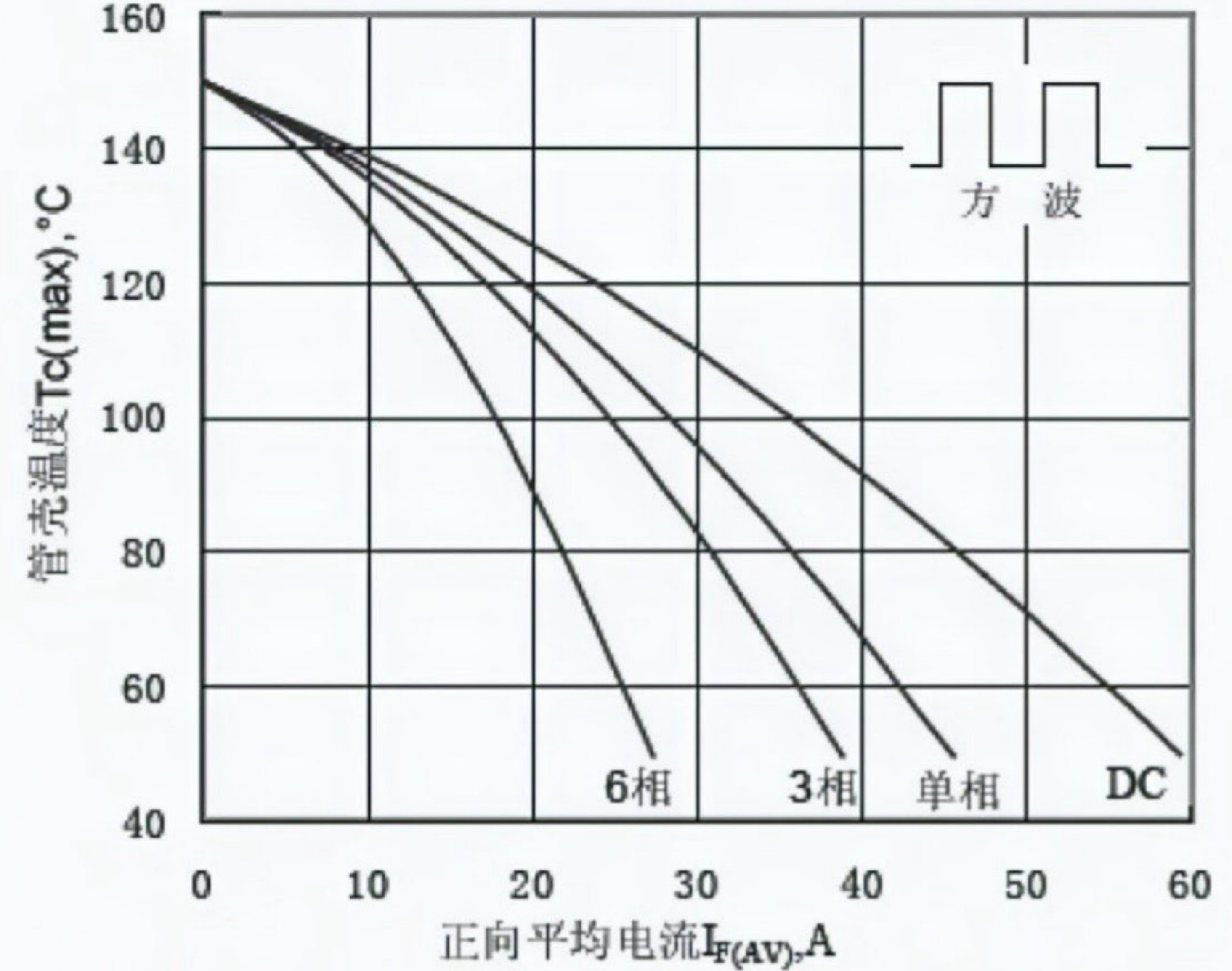
Max. case Temperature Vs. Mean forward Current
